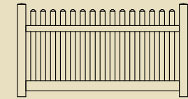
DOGEAR STRAIGHT PICKET 2"x 6" Bottom Rail 8' wide panels available 5', 4' and 3' high 6' wide panel available 4' high
