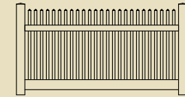
CLASSIC STRAIGHT PICKET 2"x 6" Bottom Rail 8' wide panels available 6', 5', 4' and 3' high 6' wide panel available 4' high
